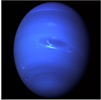
Neptune
