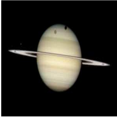
Saturne
